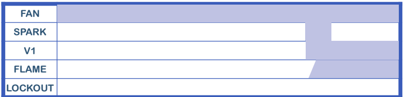
A-Start sequence, flame established
