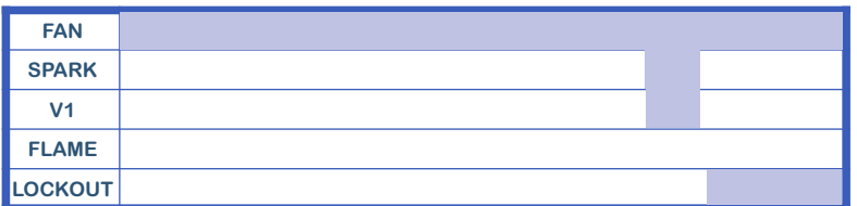
B-Start sequence, flame not established
